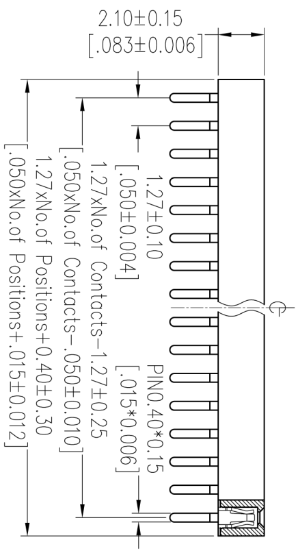
SECTION B-B
